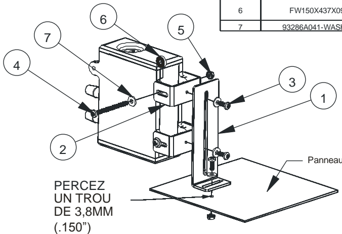
MONTAGE VERTICAL
