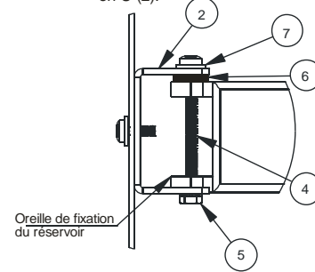
MONTAGE VERTICAL
