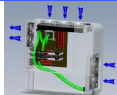
Redondance de pompe MCR320 Drive + MCR220 Drive
