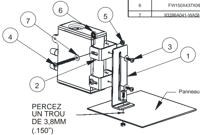
MONTAGE VERTICAL
