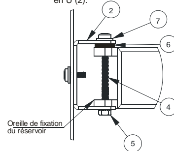
MONTAGE VERTICAL
