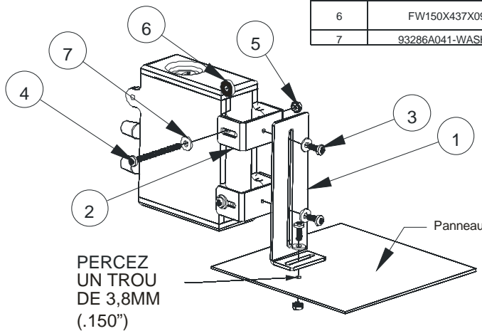
MONTAGE VERTICAL
