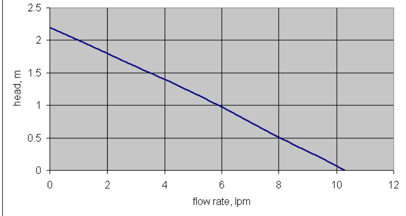
MCP600 Pump Performance Curve
