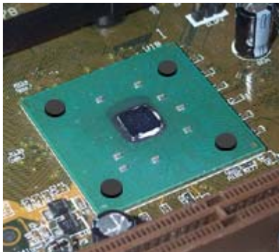
Figure 1 – Neoprene pads required
